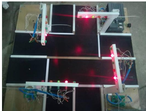
Figure 9. The Main Road is Green and Side Road is red, All Turn are OFF
